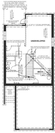
BASEMENT (UNDEV.)
