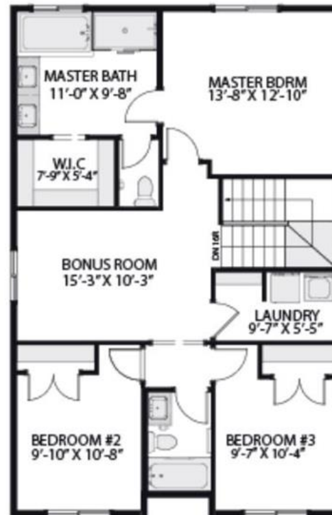
Upper Floor 1033 sqft.
