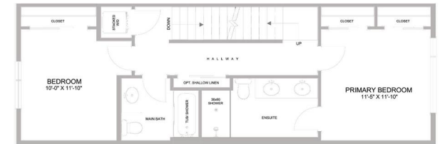
FLOORPLAN B | THIRD FLOOR
