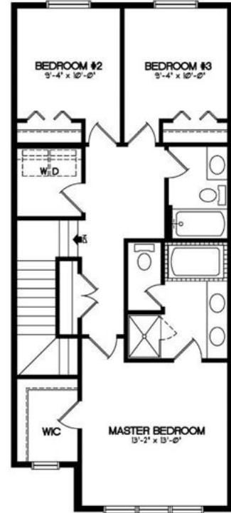
UPPER FLOOR - 835 SQFT
