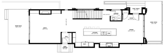
MAIN FLOOR PLAN SCALE: 3/16" = 1'-0" 10/20/2018/001
