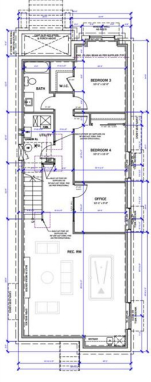
PROPOSED BSMT FLOOR PLAN
