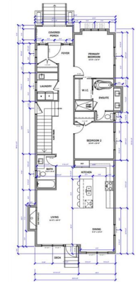
PROPOSED MAIN FLOOR PLAN
