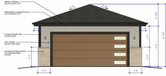
4 GARAGE (SOUTH) 1/4" = 1'-0"
