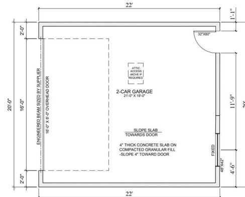
GARAGE PLAN
