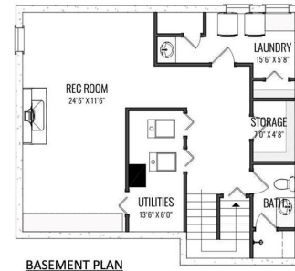
BASEMENT PLAN
