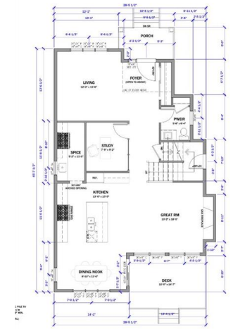
PROPOSED MAIN FLOOR PLAN SCALE: 1/4" = 1'-0" CEILING HT: 9'-0" MAIN FLOOR: 1,130 SQ.FT. SECOND FLOOR: 1,060 SQ.FT. TOTAL AREA: 2,190 SQ.FT.
