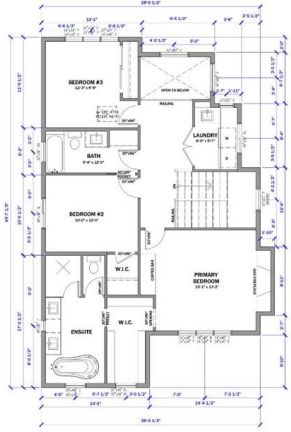
PROPOSED UPPER FLOOR PLAN SCALE: 1/4" = 1'-0" CEILING HT: 9'-0" MAIN FLOOR: 1,138 SQ.FT. SECOND FLOOR: 1,000 SQ.FT. TOTAL AREA: 2,138 SQ.FT.
